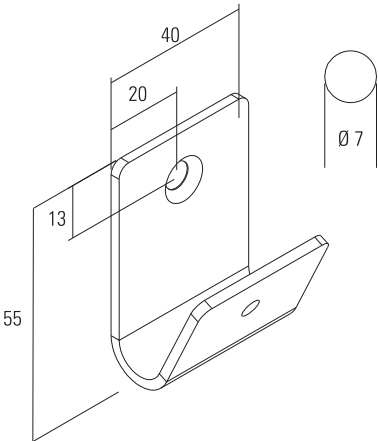
WALL BRACKET
