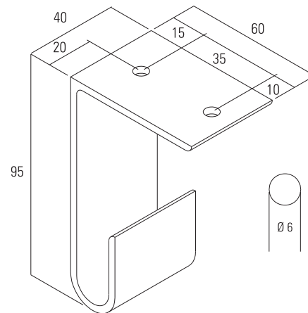
CEILING BRACKET
