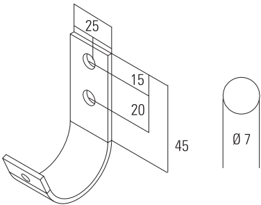
WALL BRACKET
