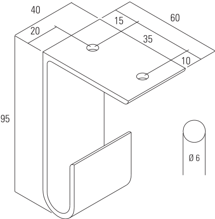
CEILING BRACKET
