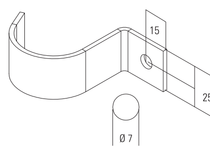
SIDE BRACKET
