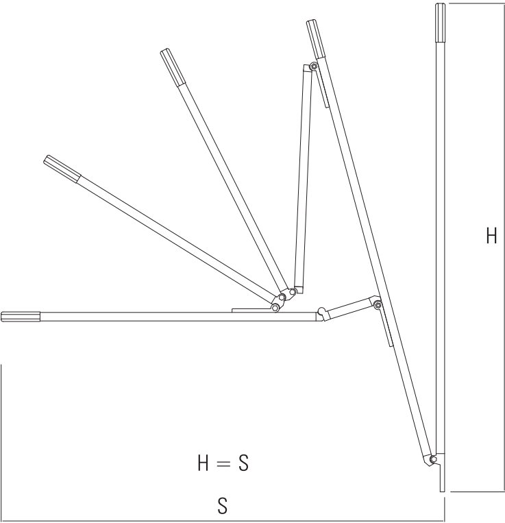
WALL BRACKET
