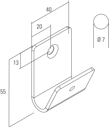
WALL BRACKET
