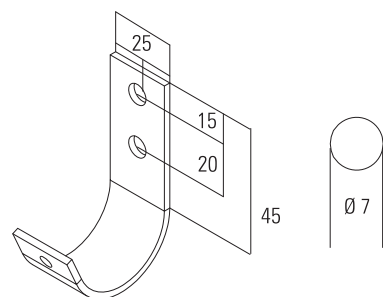
WALL BRACKET
