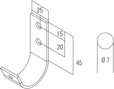
WALL BRACKET
