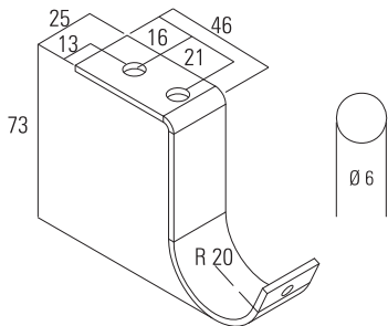
CEILING BRACKET
