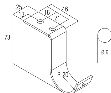
CEILING BRACKET
