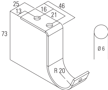
CEILING BRACKET
