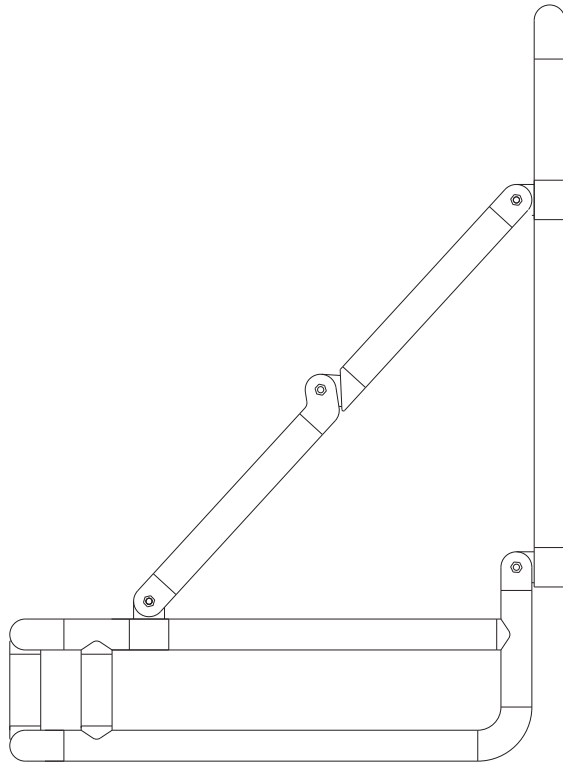
WALL BRACKET
