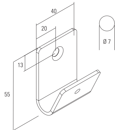
WALL BRACKET
