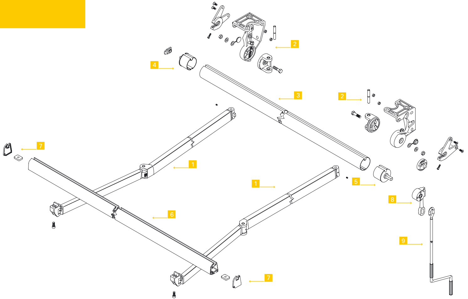
braccio Aries Plus - Aries Plus arm - Gelenkarm Aries Plus - bras Aries Plus
